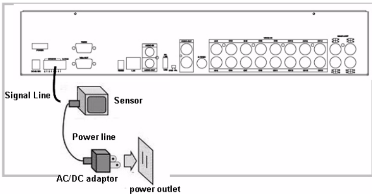
Figure 2.3: Sensor installation
