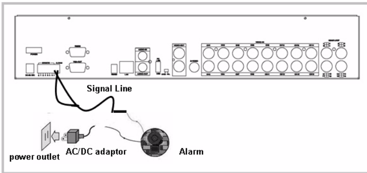
Figure 2.4: Alarm installation
