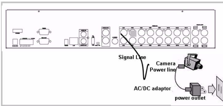
Figure 2.2: Video input connection
