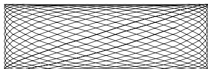
Figure 3-5 Semi-omnidirectional Scan Pattern
