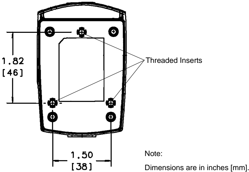
Figure 2-2 Symbol MS3204 Mounting Dimensions
