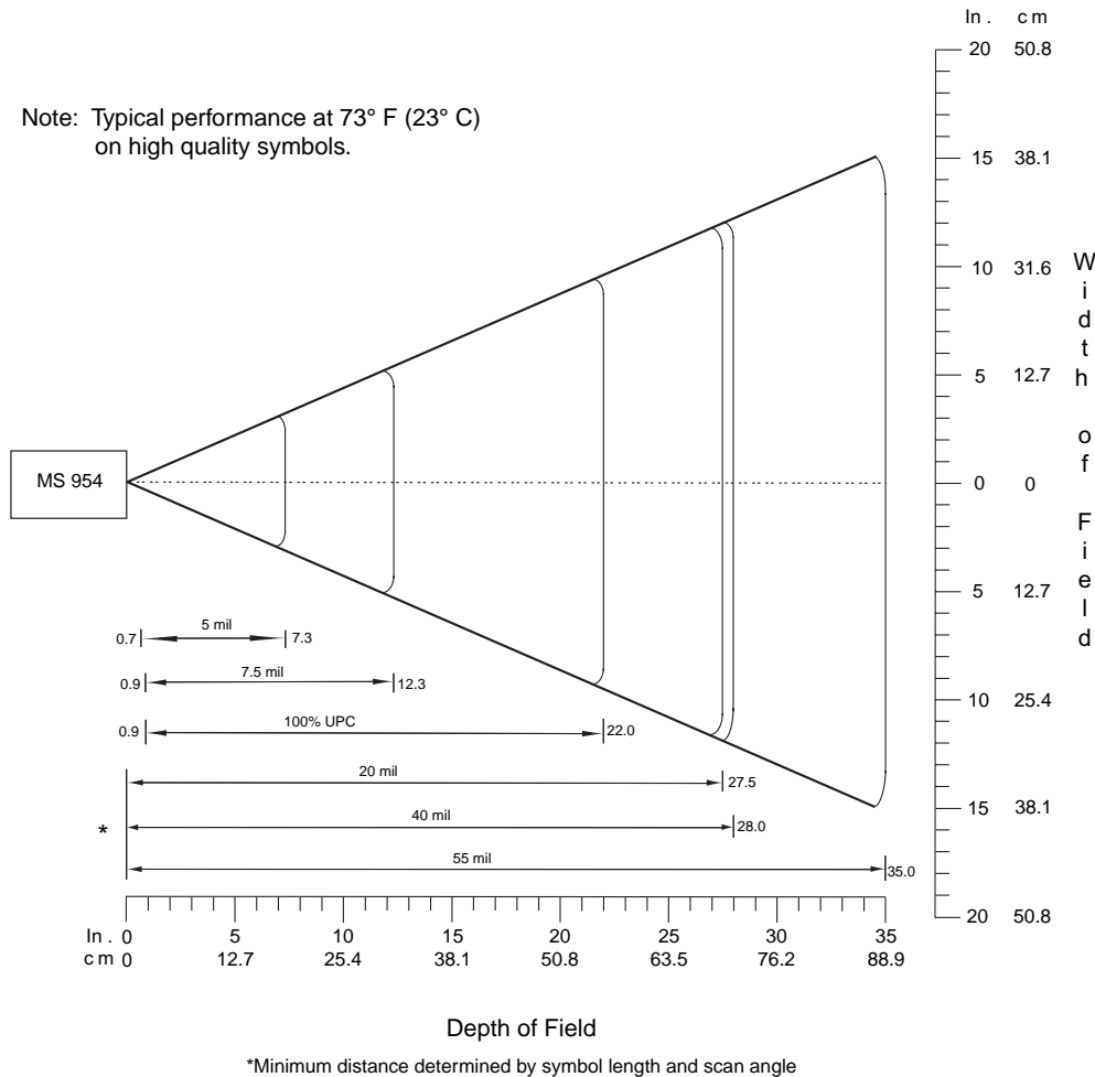
Figure 8-5 Symbol MS954 Decode Zone
