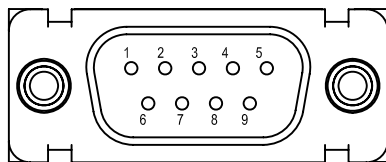
Figure 6-1 MiniScan Connector
