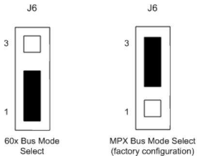
Figure 2-4 Jumper Setting for J6
