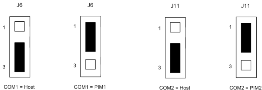
Figure 5-4 COM1 and COM2 Serial Port Jumpers (J6/J11)
