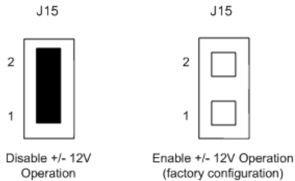
Figure 2-7 Jumper Settings for J15
