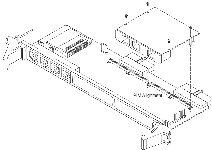
Figure 5-9 Installing the PIM
