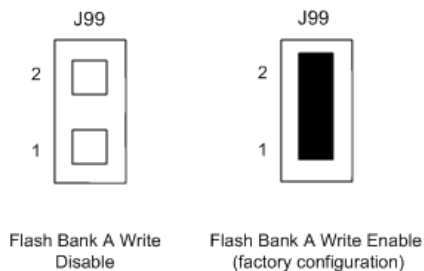
Figure 2-10 Jumper Setting for J99
