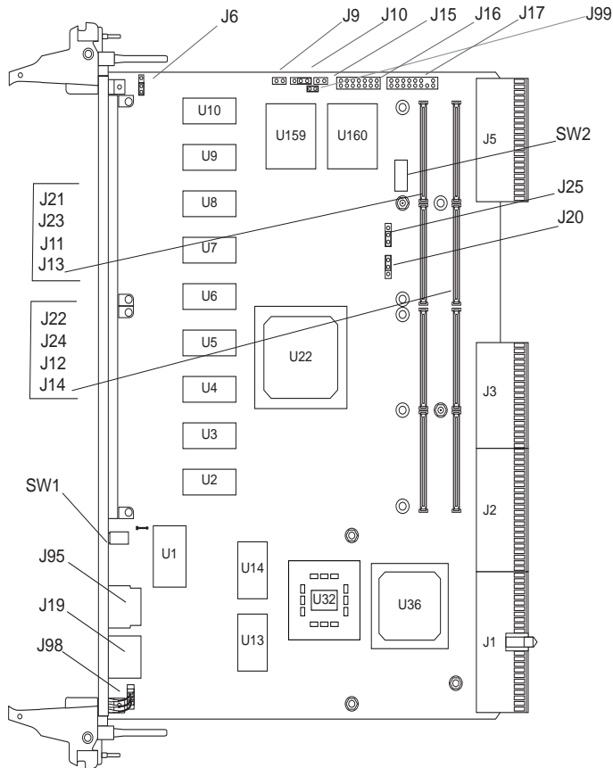
Figure 3-1 Component Layout
