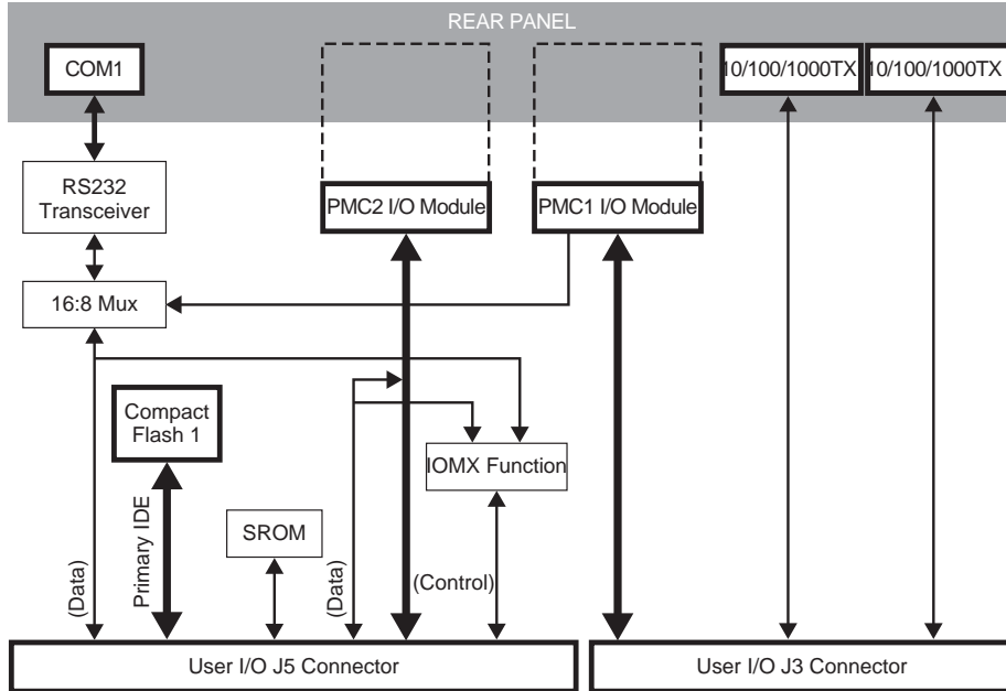
Figure 5-1 CPCI-6115-MCPTM Block Diagram
