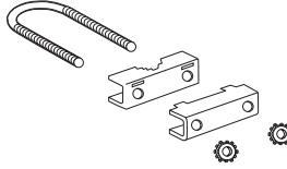
U-Bolt (1), Mast Clamp (1), Mast Clamp Back-up plate (1), Lock Nuts (2)
