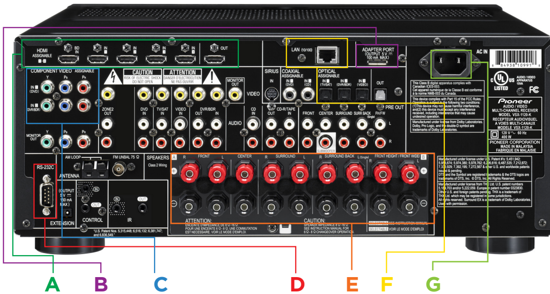
Rear Panel
