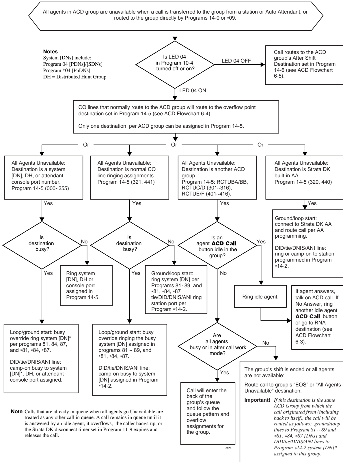
Flowchart 6-6 All Agents Unavailable Operation
