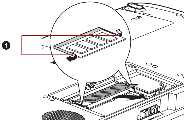
Figure 3-7 Removing the memory module
