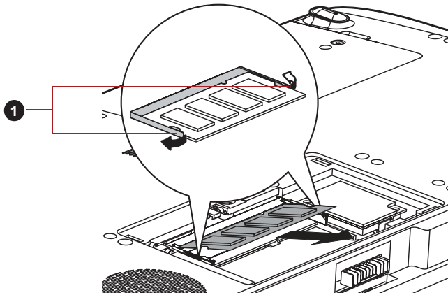
Figure 3-7 Removing the memory module
