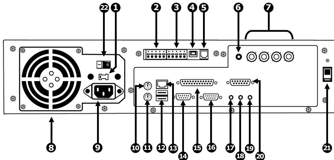
Figure 1.3 KV-KLR Rear
