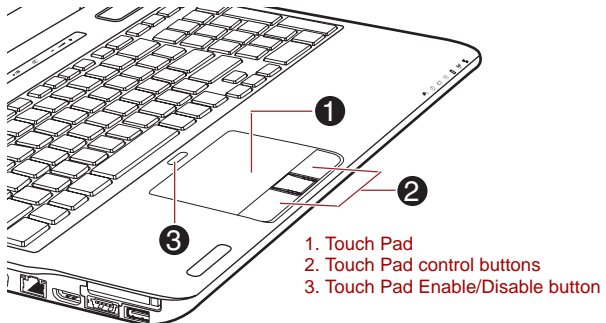
Figure 4-1 Touch Pad and Touch Pad control buttons
