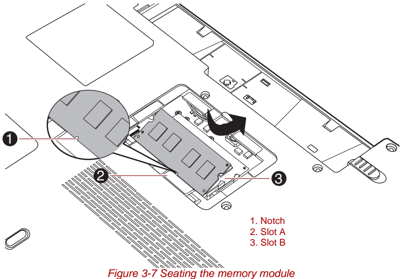
Figure 3-7 Seating the memory module
