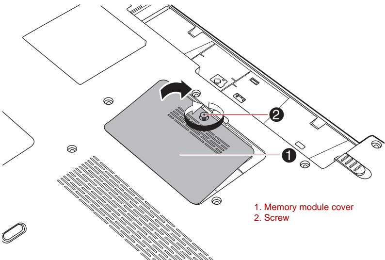
Figure 3-8 Seating the memory module cover
