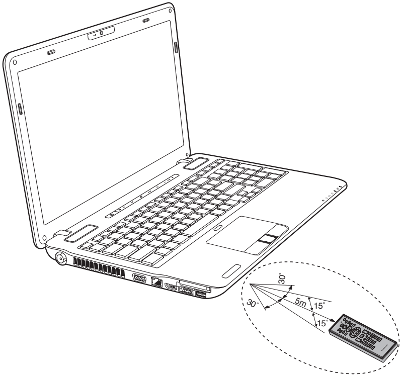
Figure 2-12 Operational range of the remote control
