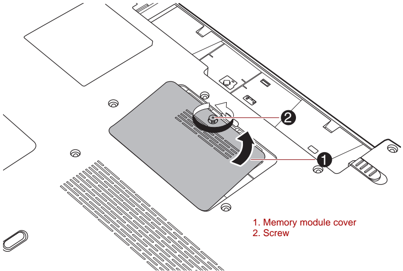
Figure 3-6 Removing the memory module cover
