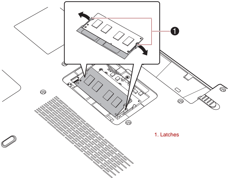
Figure 3-9 Removing the memory module
