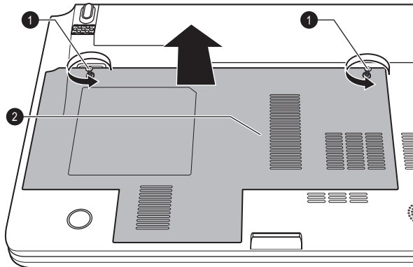
Figure 3-7 Removing the memory module cover
