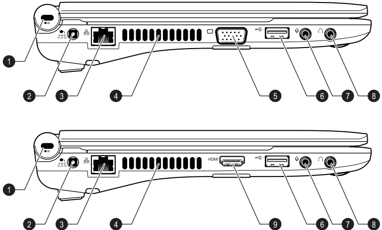
Figure 2-2 The left side of the computer
