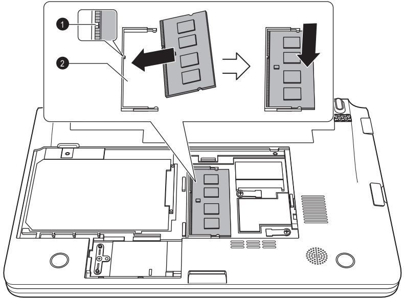
Figure 3-8 Seating the memory module
