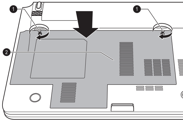
Figure 3-9 Seating the memory module cover
