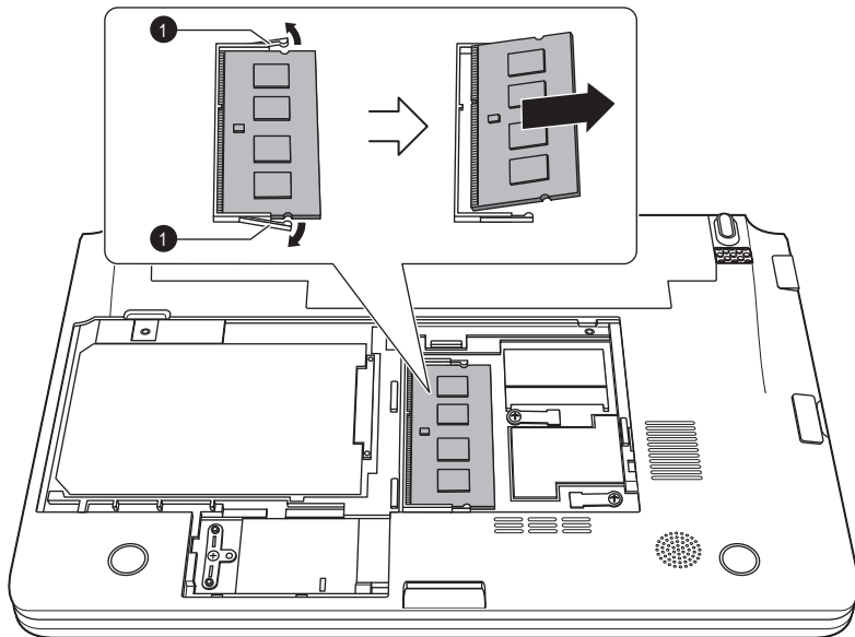
Figure 3-10 Removing the memory module
