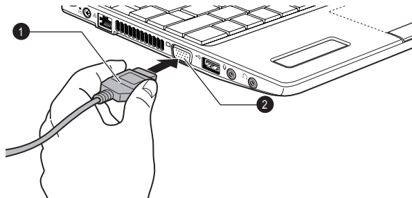
Figure 3-11 Connecting the monitor cable to the external monitor port
