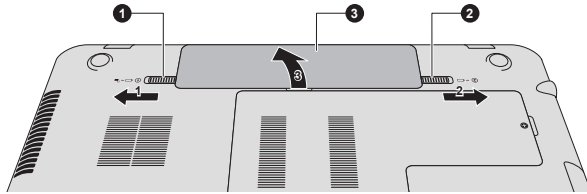
Figure 4-11 Releasing the battery pack -2
