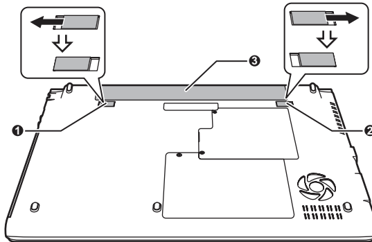
Figure 5-1 Releasing the battery pack (R830)
