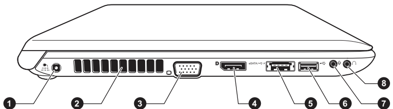
Figure 2-8 The left side of the computer (R840)
