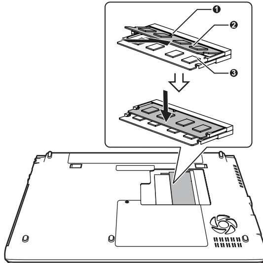
Figure 3-13 Seating the memory module (R830)
