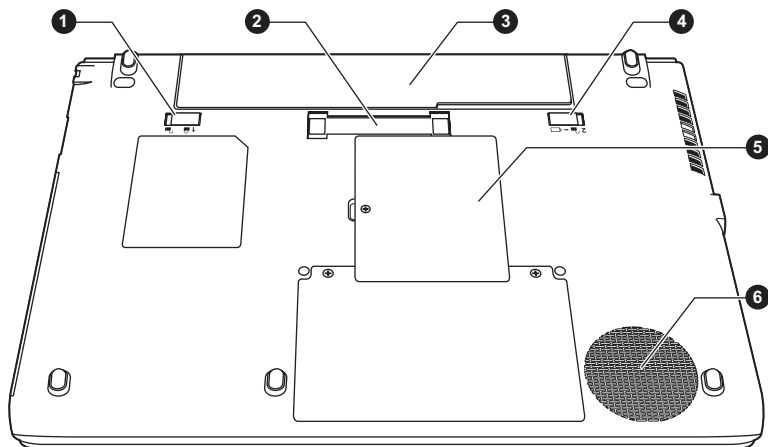
Figure 2-11 The underside of the computer (R840)
