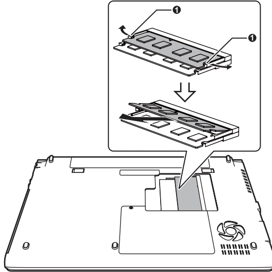
Figure 3-15 Removing the memory module (R830)
