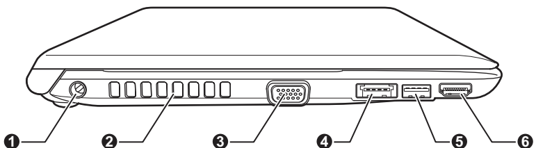
Figure 2-14 The left side of the computer (R830)
