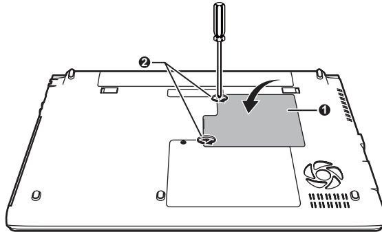
Figure 3-14 Seating the memory module cover (R830)
