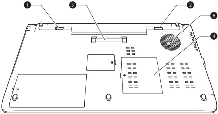
Figure 2-5 The underside of the computer (R850)
