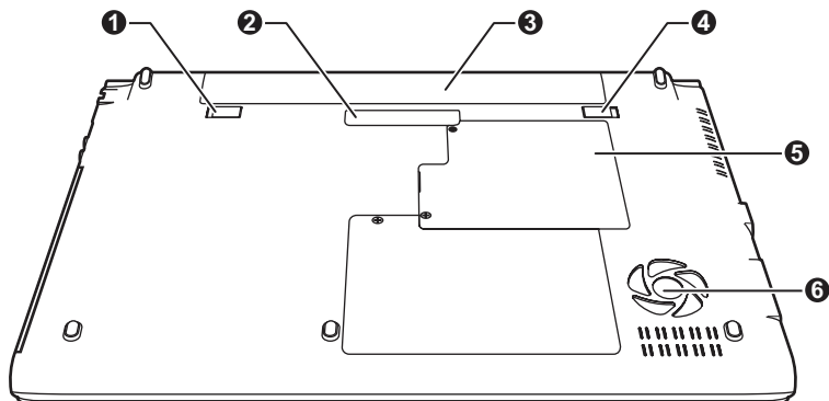
Figure 2-17 The underside of the computer (R830)
