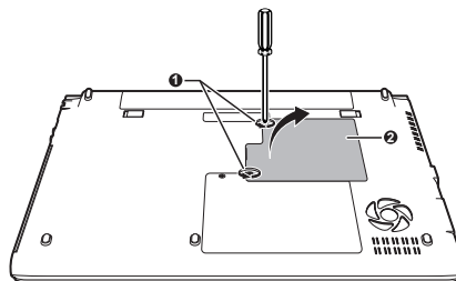
Figure 3-14 Removing the memory module cover (R830)
