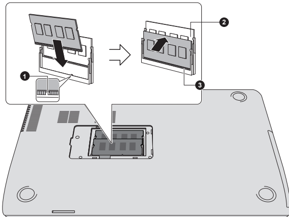
Figure 4-7 Seating the memory module
