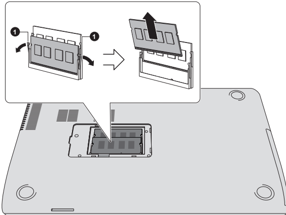
Figure 4-9 Removing the memory module
