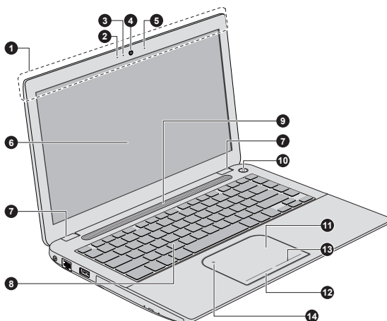
Figure 3-6 The front of the computer with the display panel open(non-touch model)
