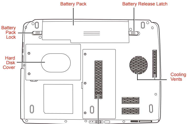
Memory Module and Wireless LAN Cover The underside of the computer
