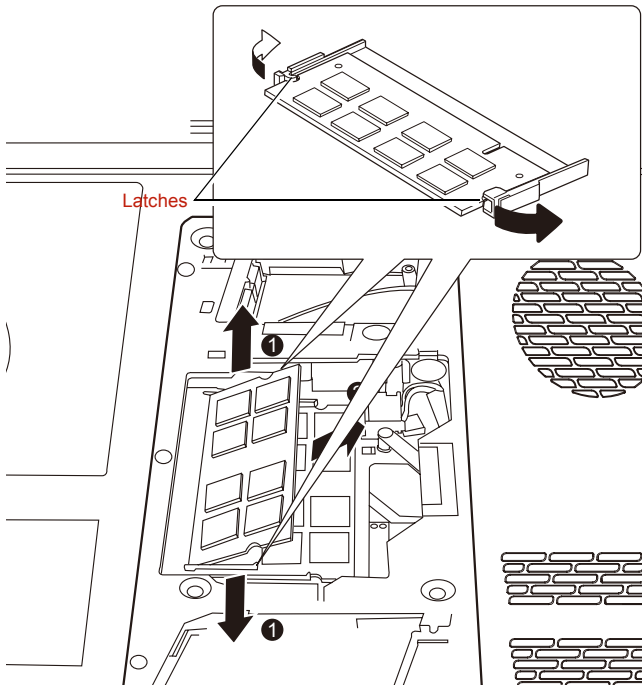
Removing the memory module
