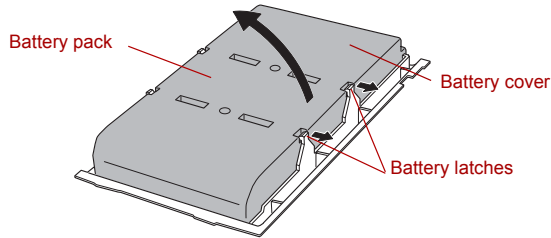
Figure 6-2 Separating the battery pack and battery cover
