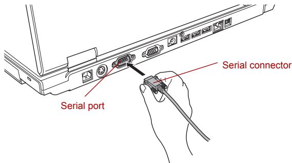
Figure 8-18 Connecting the serial connector to the serial port
