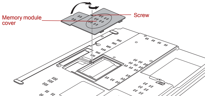
Figure 8-5 Removing the memory module cover
