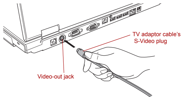
Figure 8-16 Connecting the S-Video cable to the Video-out jack
