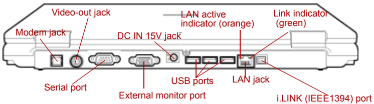
Figure 2-4 The back side of the computer
