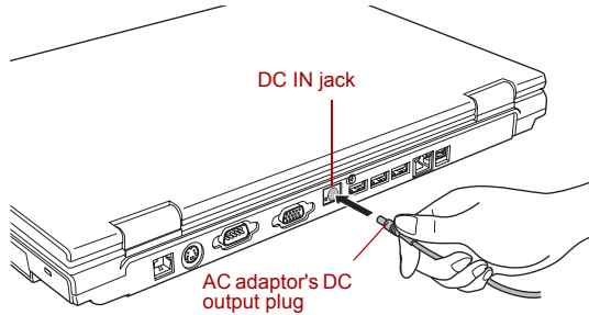
Figure 3-4 Connecting the adaptor to the computer
