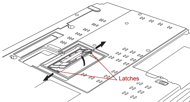
Figure 8-8 Removing the memory module
