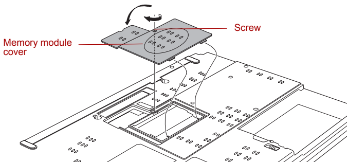
Figure 8-7 Seating the memory module cover
