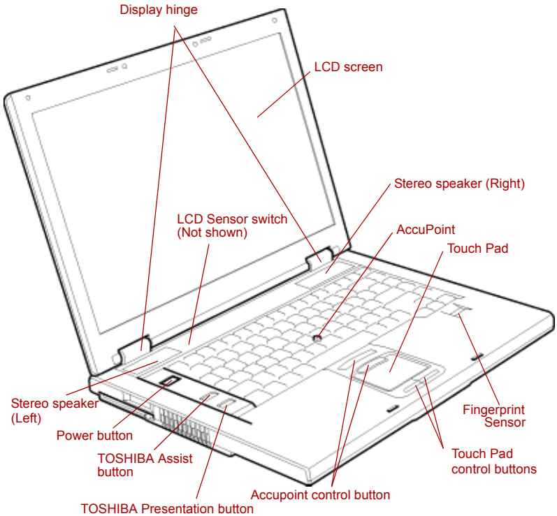
Figure 2-6 The front of the computer with the LCD display panel open
