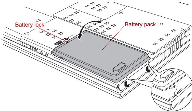
Figure 6-3 Securing the battery pack
