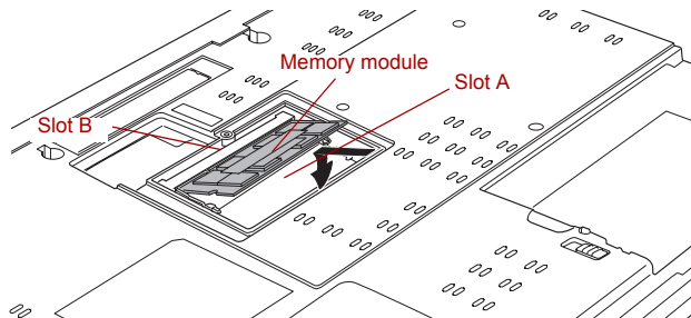
Figure 8-6 Seating the memory module
