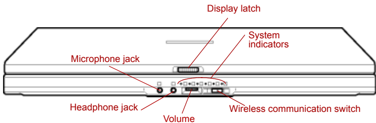
Figure 2-1 Front of the computer with LCD display panel closed
