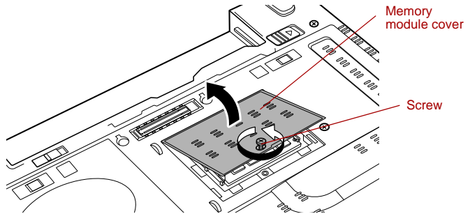
Figure 3-8 Removing the memory module cover
