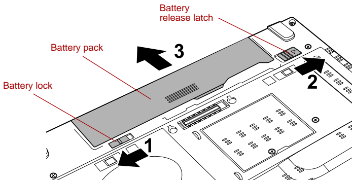
Figure 6-1 Releasing the battery pack
