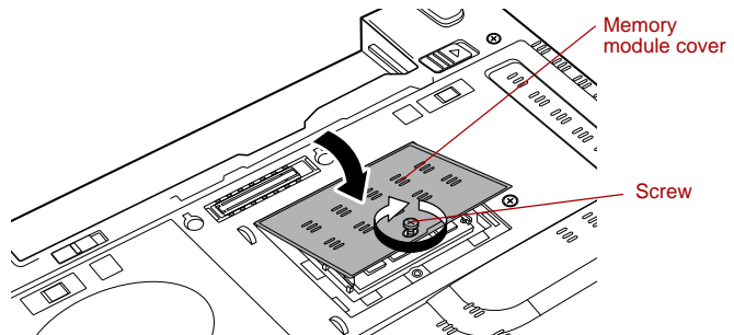
Figure 3-10 Seating the memory module cover
