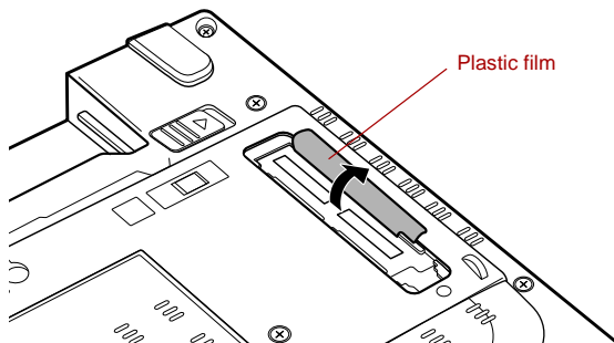
Figure G-2 Lift the plastic film
