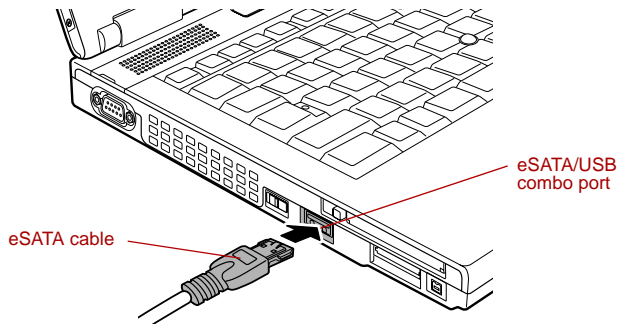
Figure 3-15 Connecting an eSATA cable to the eSATA/USB combo port
