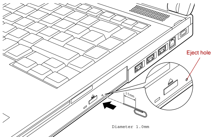
Figure 4-9 Manual release with the eject hole
