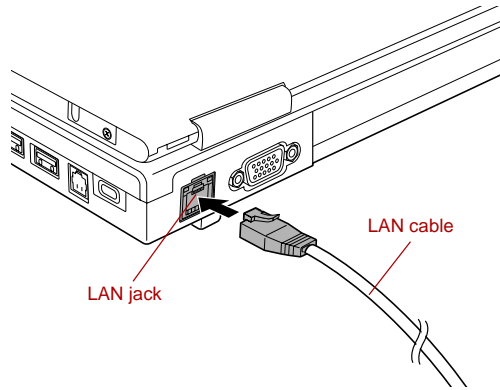
Figure 4-11 Connecting the LAN cable
