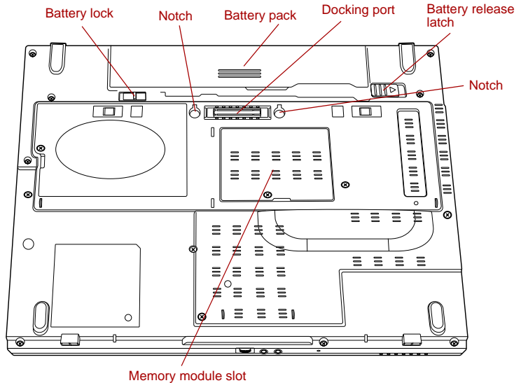
Figure 2-5 The underside of the computer
