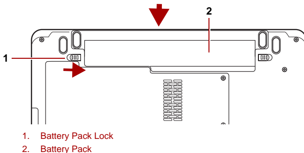
Figure 6-3 Securing the battery pack
