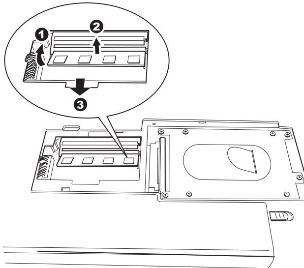
Figure 8-7 Removing the memory module
