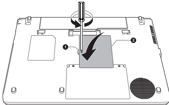
Figure 3-14 Seating the memory module cover (R940)
