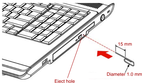
Figure 4-3 Manual release with the eject hole
