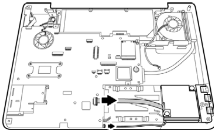
Figure 4-55 Disconnecting the USB board cable and subwoofer cable
