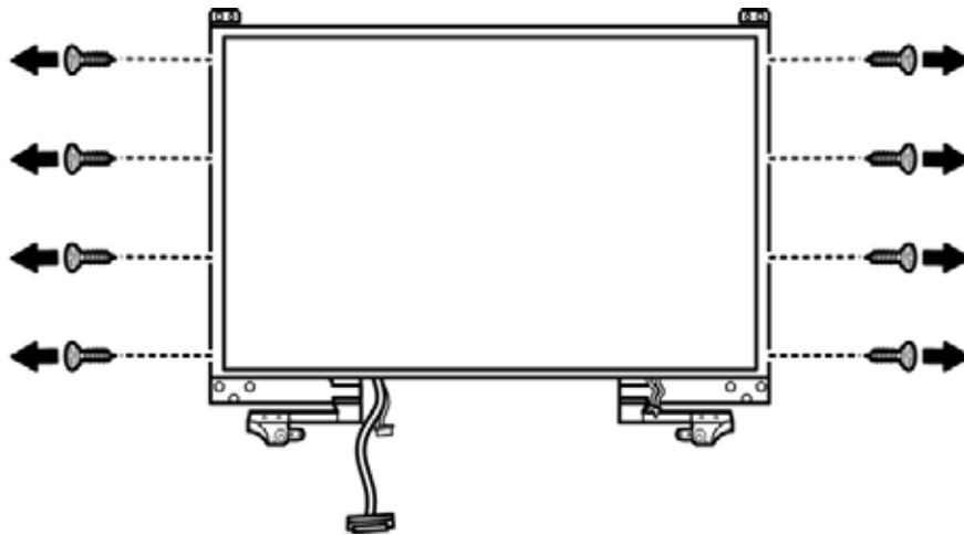
Figure 4-83 Removing the bracket screws
