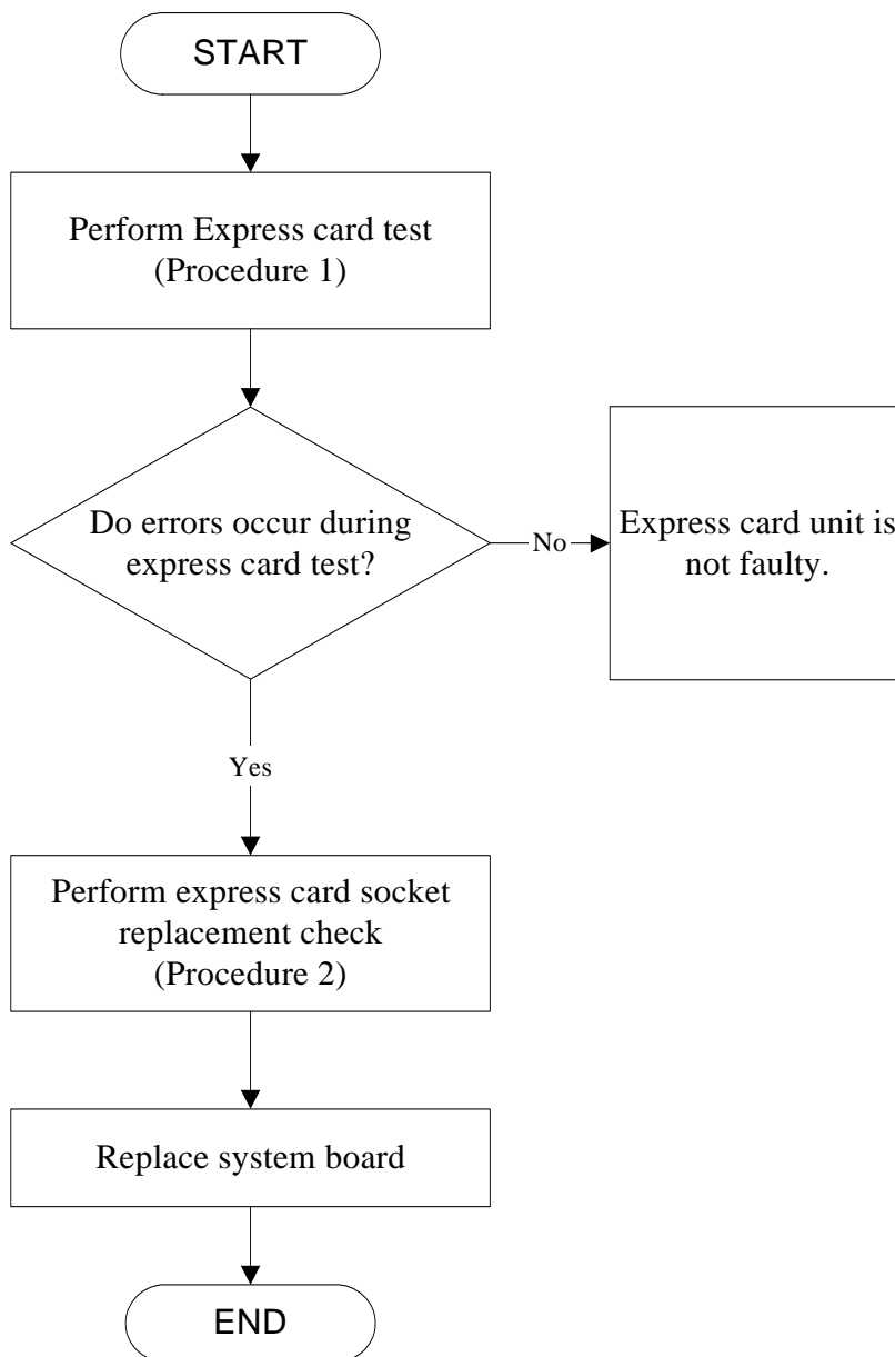
Figure 2-11 Express card troubleshooting process
