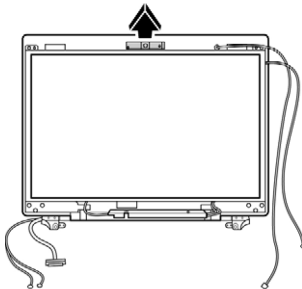
Figure 4-86 Removing the camera module
