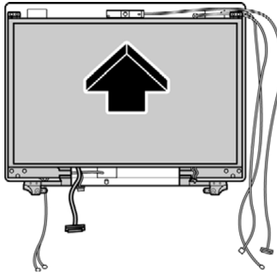
Figure 4-82 Removing the LCD Module
