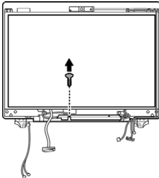
Figure 4-78 Removing the FL inverter board screws
