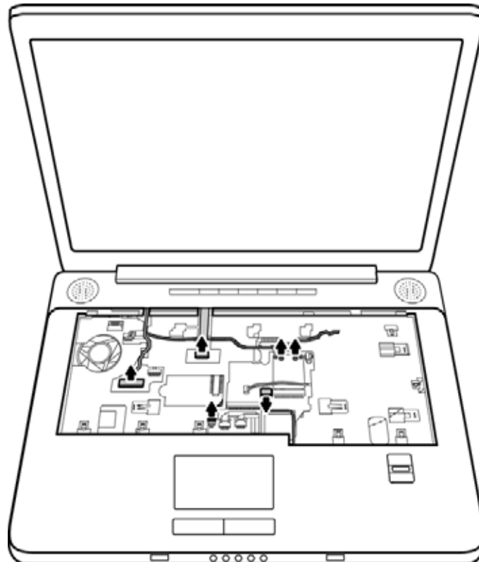
Figure 4-30 Disconnecting cables
