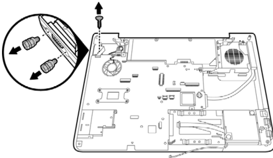
Figure 4-62 Removing the VGA PCB screw and the hexagonal screws
