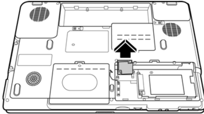
Figure 4-22 Removing the modem module
