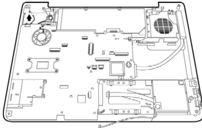
Figure 4-61 Removing the VGA PCB FFC cable
