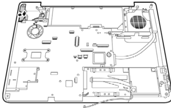
Figure 4-63 Removing the VGA PCB
