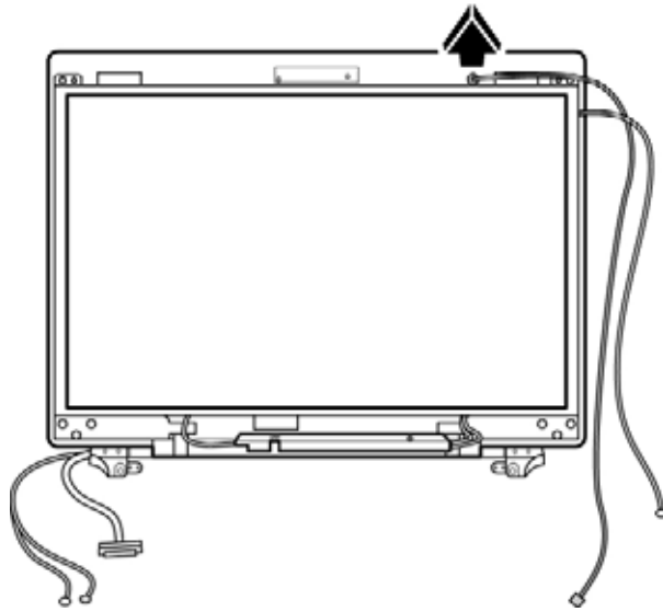
Figure 4-87 Removing the microphone
