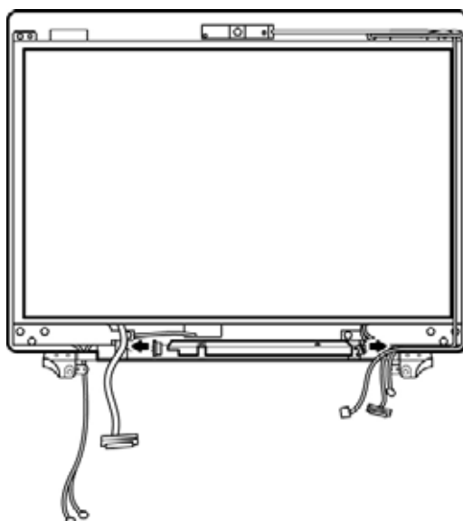
Figure 4-79 Removing the connectors
