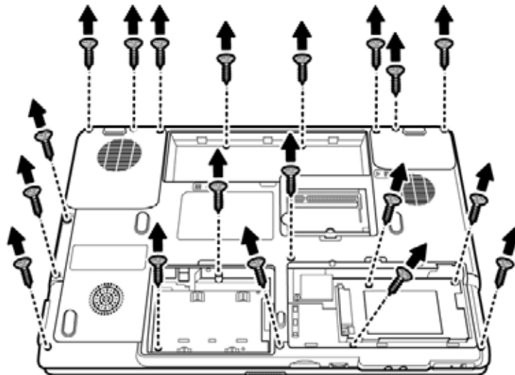
Figure 4-42 Removing the top cover (back panel screws)
