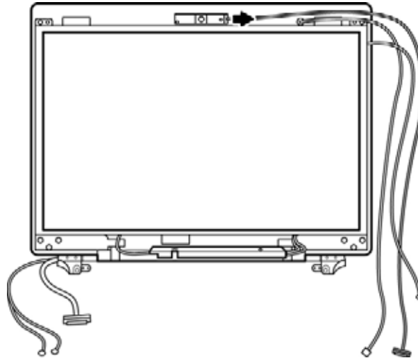
Figure 4-85 Removing the CMOS cable
