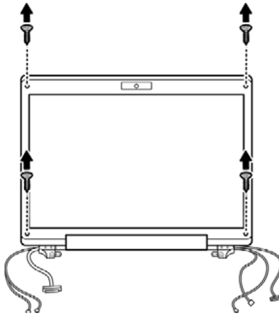
Figure 4-76 Removing the display mask screws
