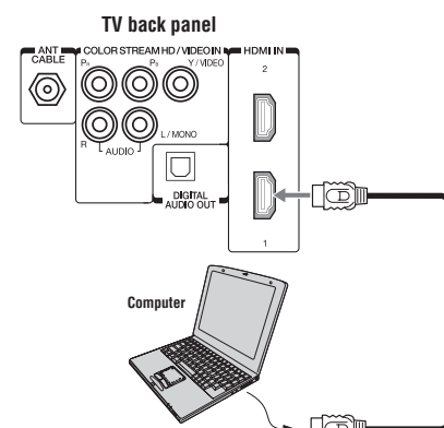
(Sample Illustration) Computer connections
