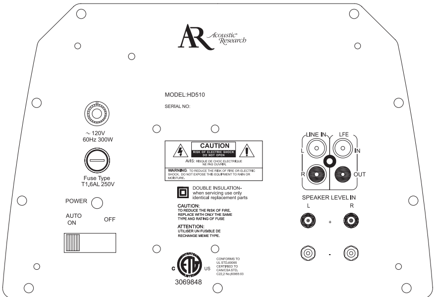
FIGURE 3 - Subwoofer Controls & Connections
