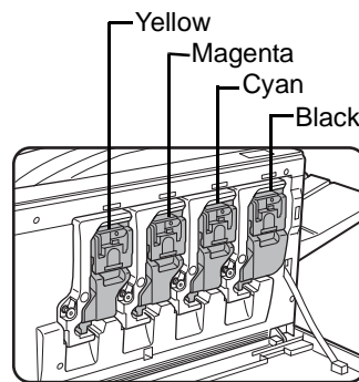
Arrangement of colour toner cartridges
