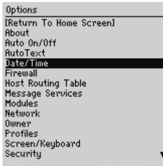
Options screen
