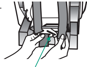
Strap Connector
