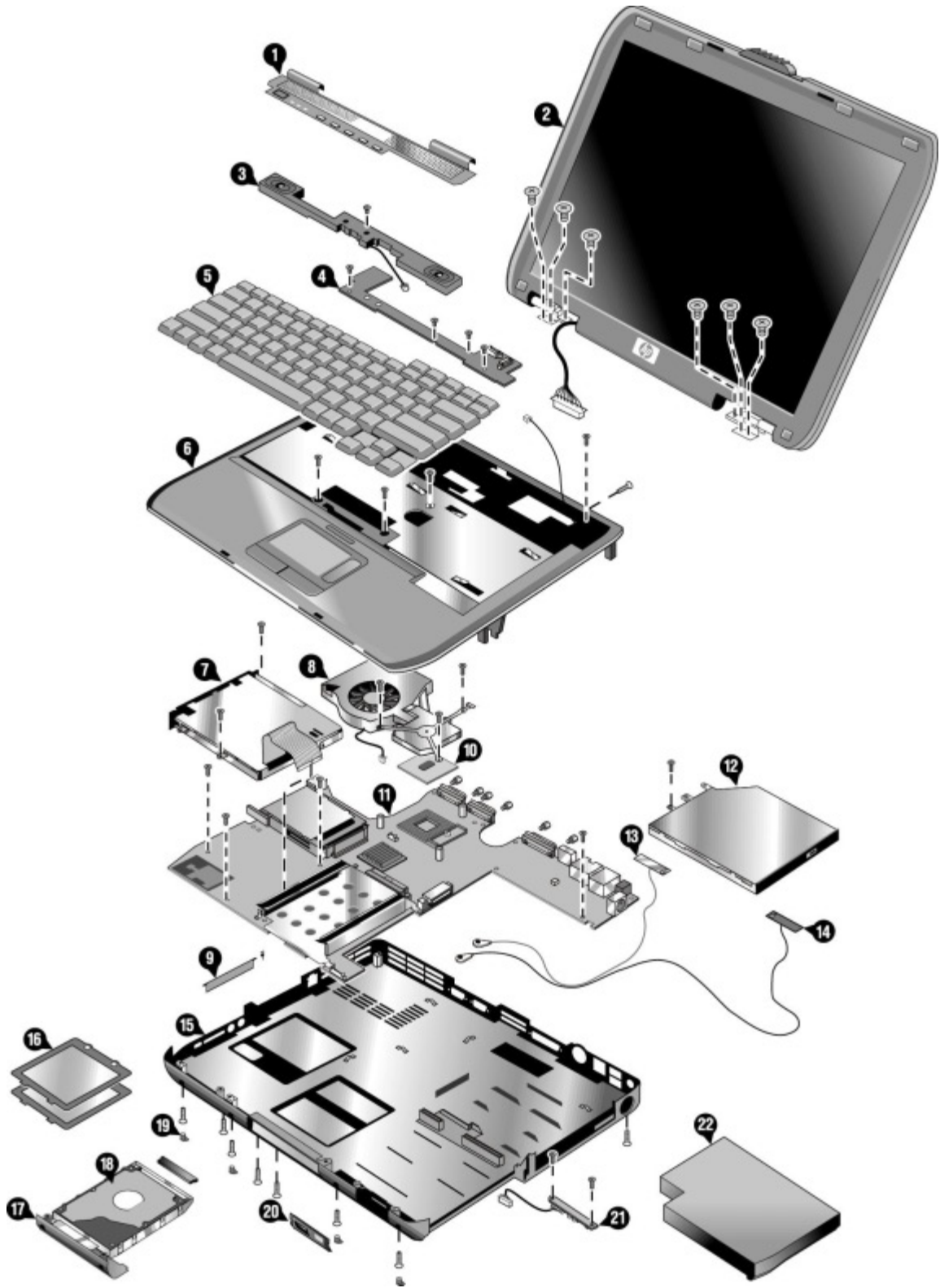
Figure 4-1. Exploded View
