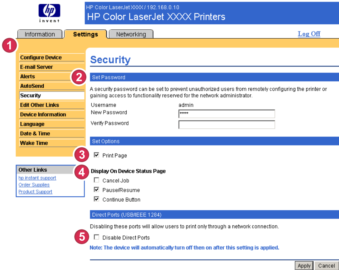
Figure 3-7 Security screen
