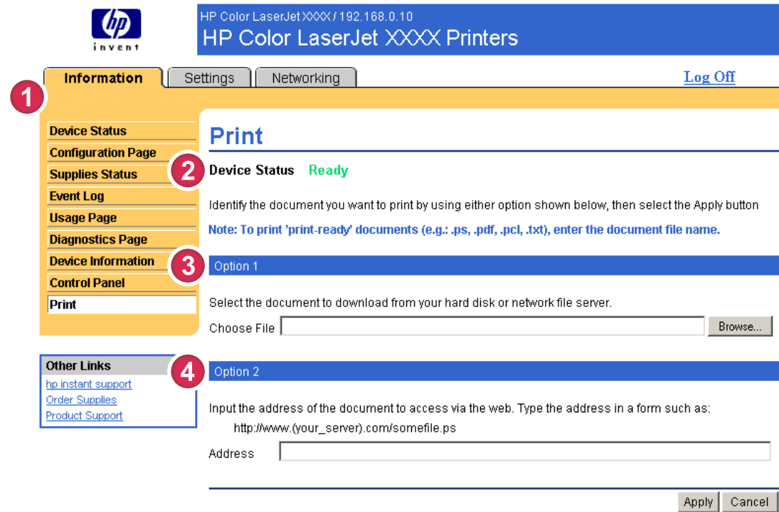
Figure 2-9 Print screen
