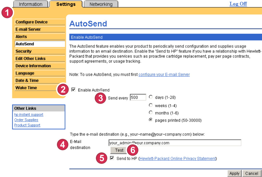
Figure 3-6 AutoSend screen
