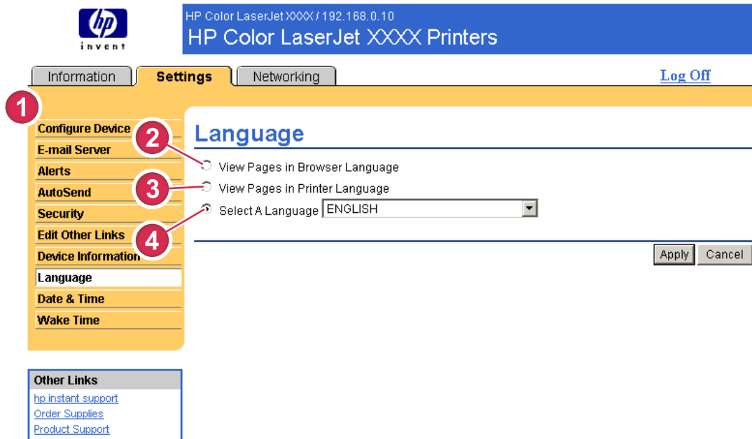
Figure 3-10 Language screen
