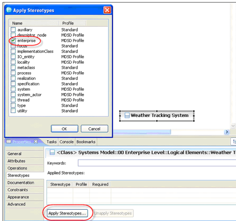
Figure 6-32 Apply stereotype
