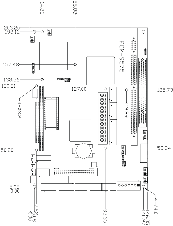
Figure 1.1: Board layout: dimensions
