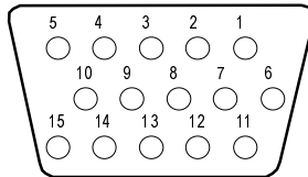
VGA/SVGA connector (Model 65E, rear panel)
