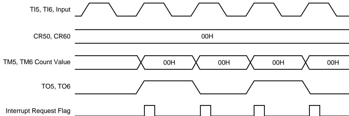
Figure 6-19. External Event Counter Operation Timing
