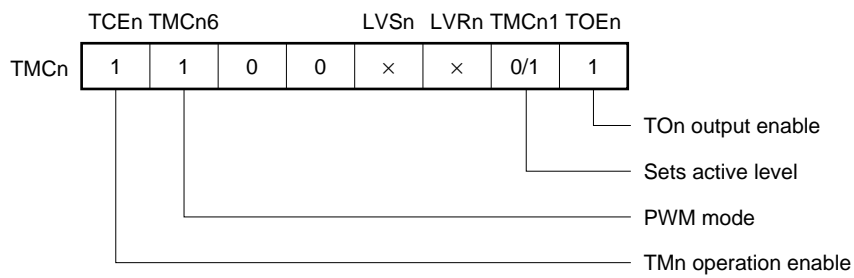
Figure 6-13. 8-Bit Timer Mode Control Register Settings for PWM Output Operation
