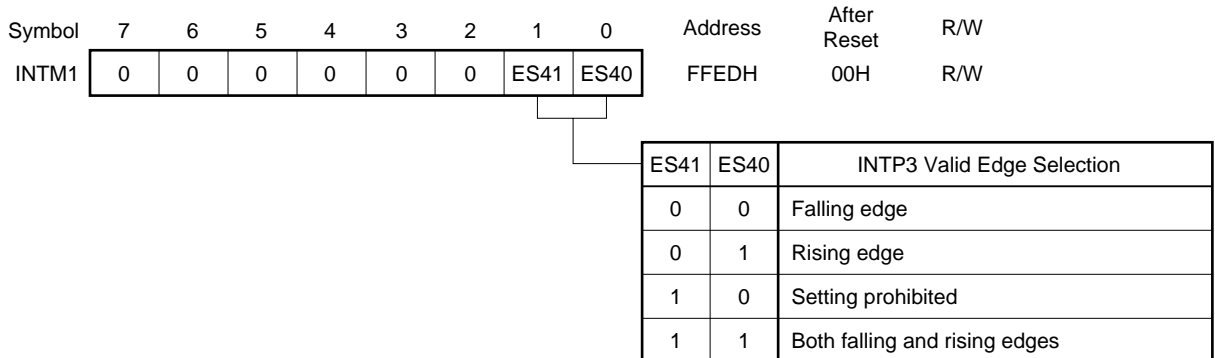
Figure 12-6. External Interrupt Mode Register 1 Format
