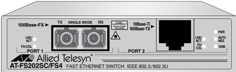
Figure 2 AT-FS202SC/FSx Series Front Panel (AT-FS202SC/FS4 Model)
