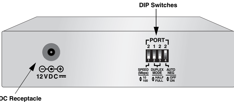
Figure 3 Back Panel of the AT-FS20x and AT-FS202SC/FSx Series Switches
