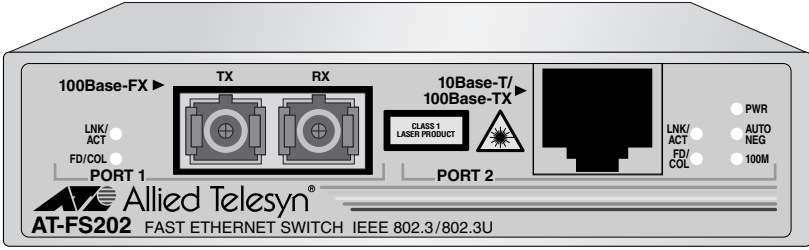
Figure 1 AT-FS20x Series Front Panel (AT-FS202 Model)
