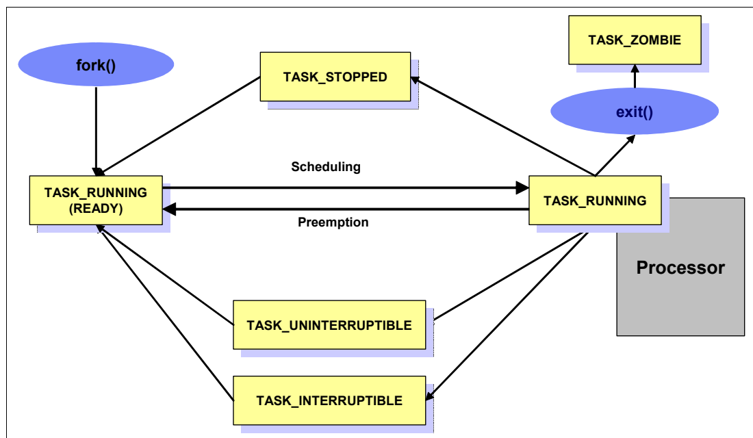
Figure 1-6 Process state
