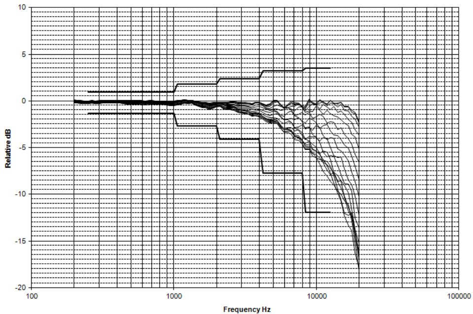
Directional frequency response positioned with a remote preamp (0°-180° incidence angles)
