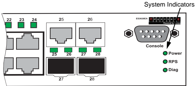
Figure 1-3 System LEDs
