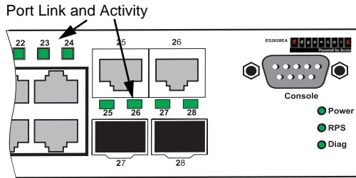
Figure 1-2 Port LEDs
