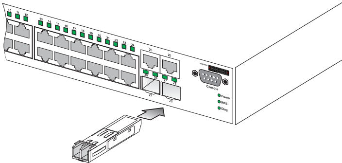
Figure 3-5 Inserting an SFP Transceiver into a Slot
