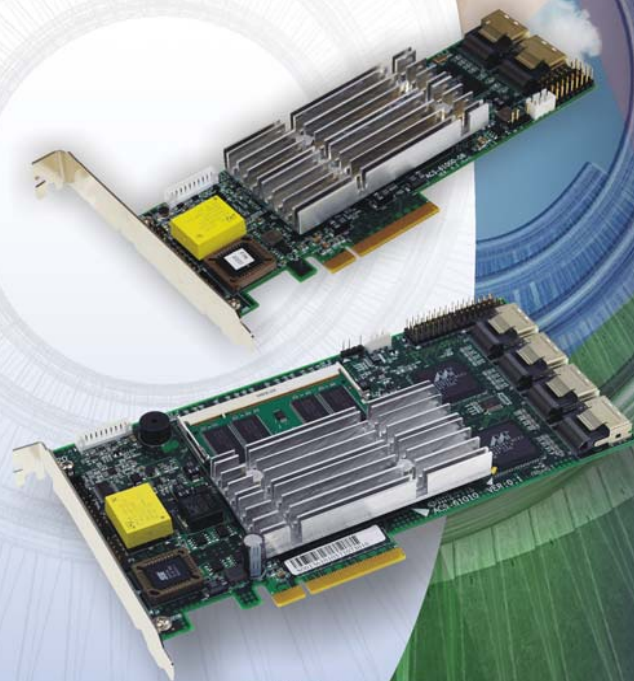
RAID Card
