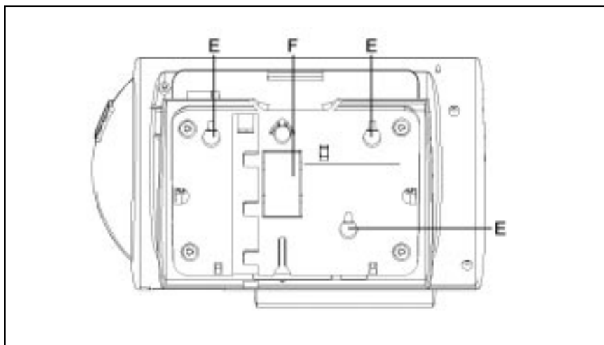
Figure 1 - M6320 wall mounting positions
