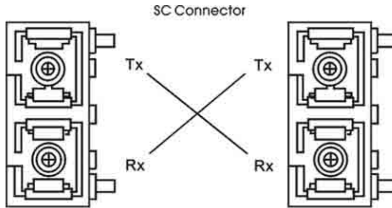
Cable Wiring(SC to SC)
