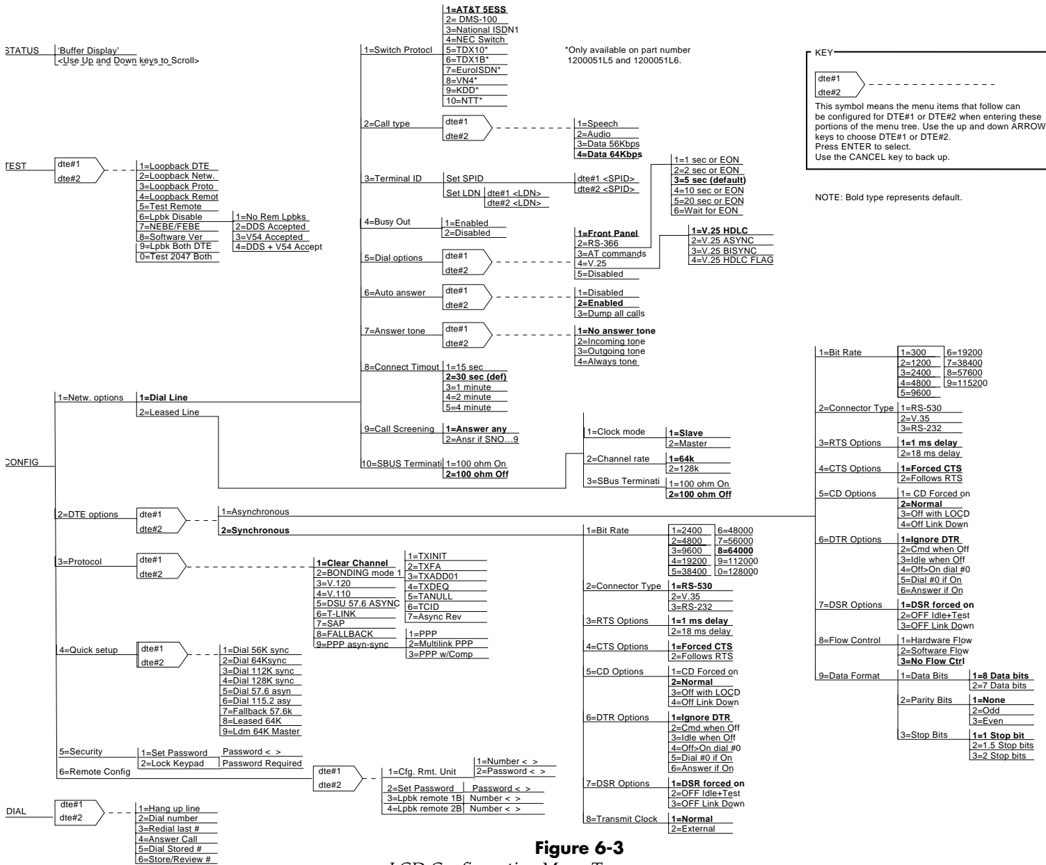
LCD Configuration Menu Tree
