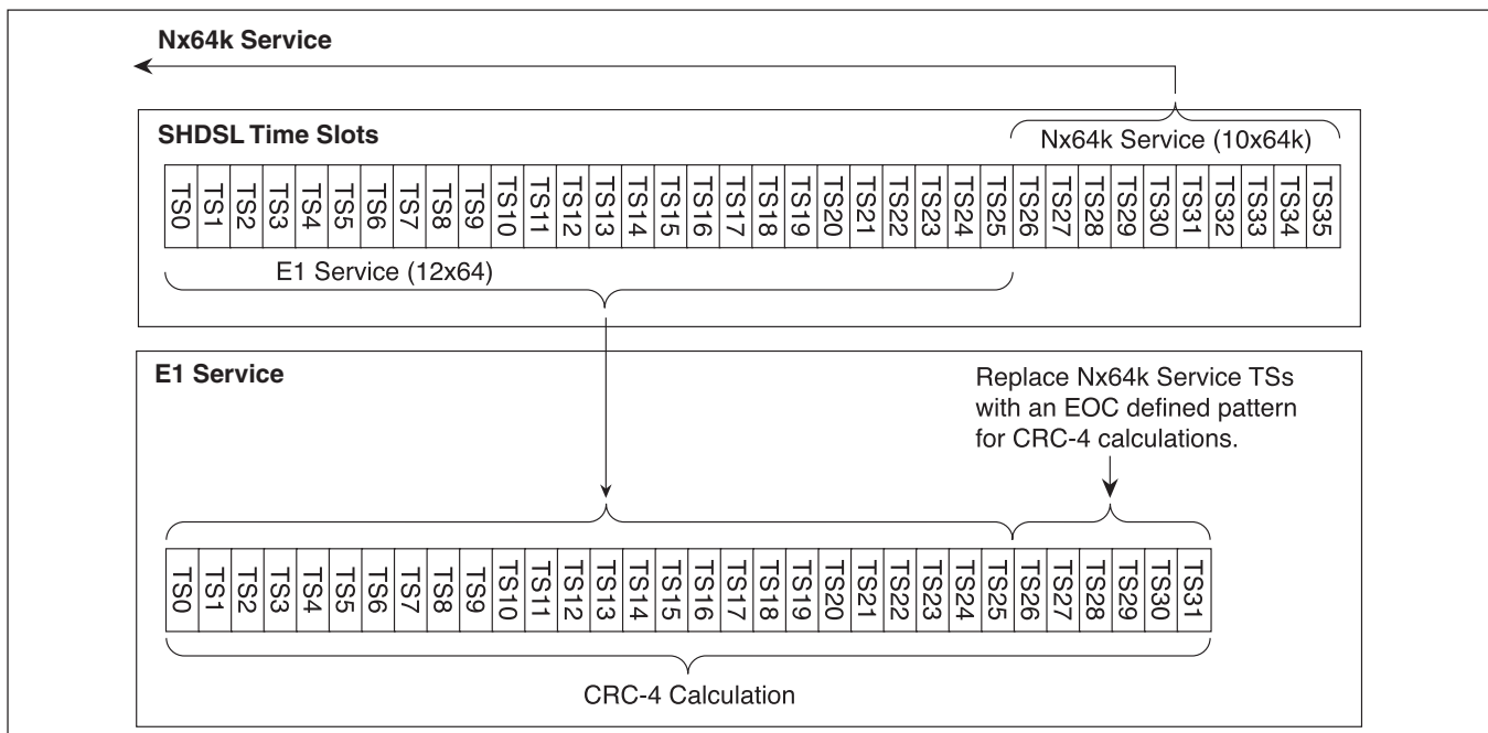
Figure 22. CRC-4 Detection/Generation
