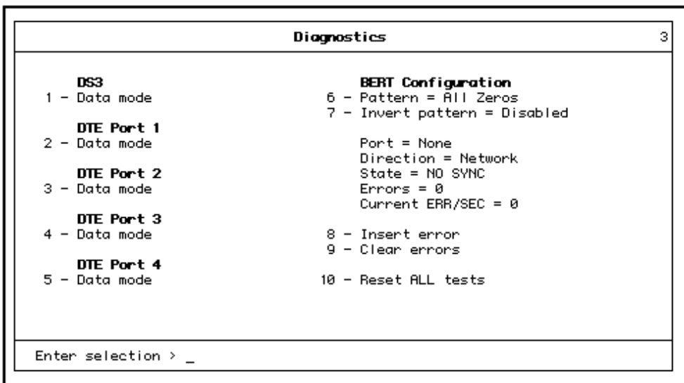
Figure 6-1. Diagnostics Main Menu
