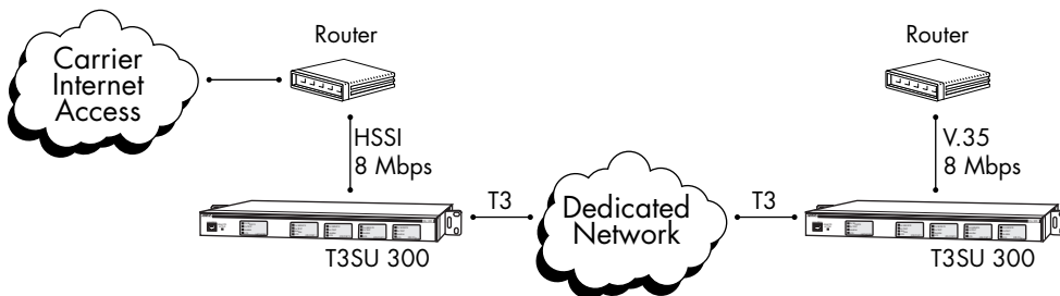
Figure 7-3. Fractional Application
