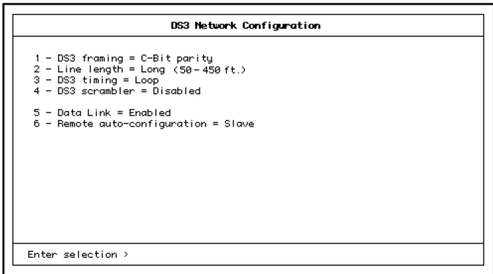
Figure 3-2. DS3 Network Configuration Menu
