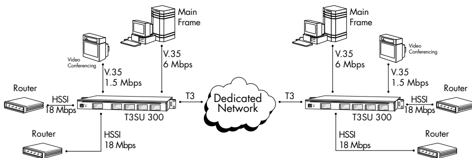
Figure 7-2. Multipoint Application
