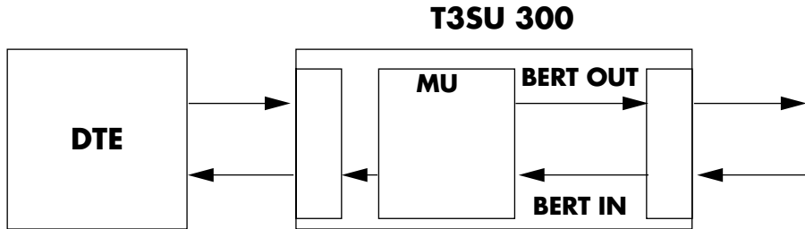
Figure 6-7. Payload BERT Test
