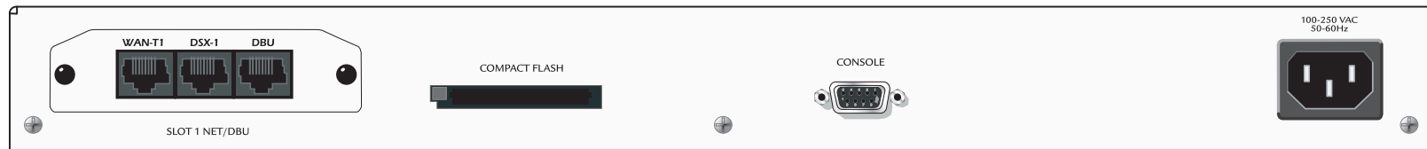
NETVANTA 1335 REAR PANEL LAYOUT
