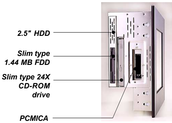
Figure 2-1: Side view
