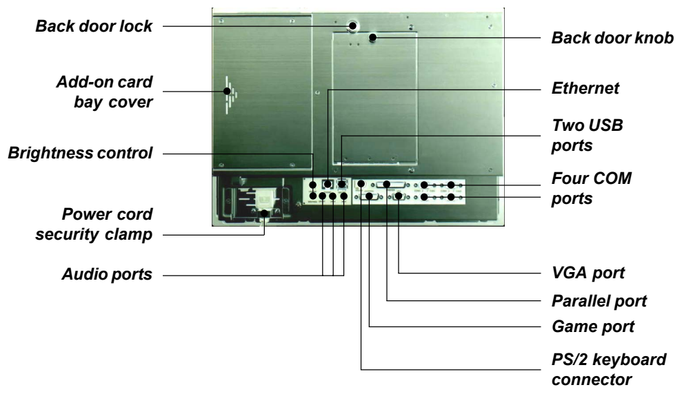
Figure 2-2: Rear view
