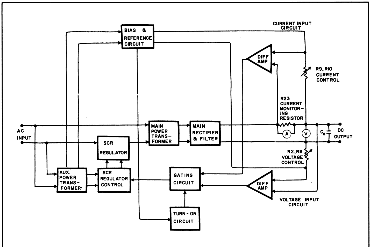
Figure 4-1. Block Diagram
