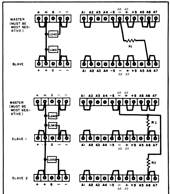
Figure 3-11. Auto-Tracking, Two and Three Units
