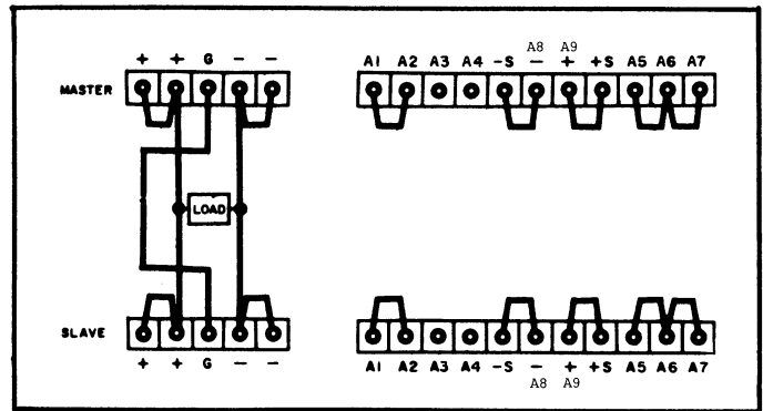
Figure 3-7. Normal Parallel Connections
