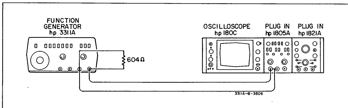
Figure 5-1. Amplitude Flatness.
