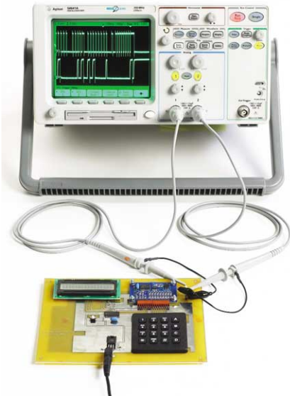
Figure 8. Trigger on address and/or data patterns within an I 2 C frame.
